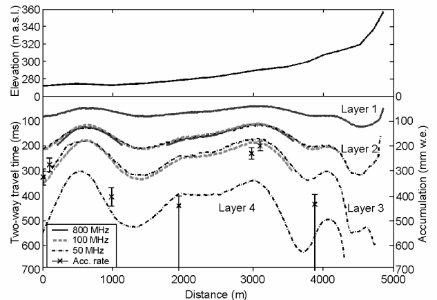
Fig. 4. Four layers seen in the radar profiles (Fig. 3): 800 MHz data shown as solid lines in dark grey, 100 MHz data as dashed lines in light grey, and 50 MHz data as dash-dot lines in black. Layer 1 (top) is seen only in 800 MHz data; layer 2 in all data; layer 3 in 50 and 100 MHz data; and layer 4 only in 50 MHz data. The accumulation rates derived from the snow pits and stake measurements are shown as black squares with the error bars. Surface topography along the profile is shown at the top.
